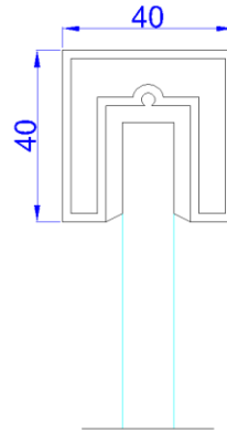
HRA40X40 SQUARE HANDRAIL
